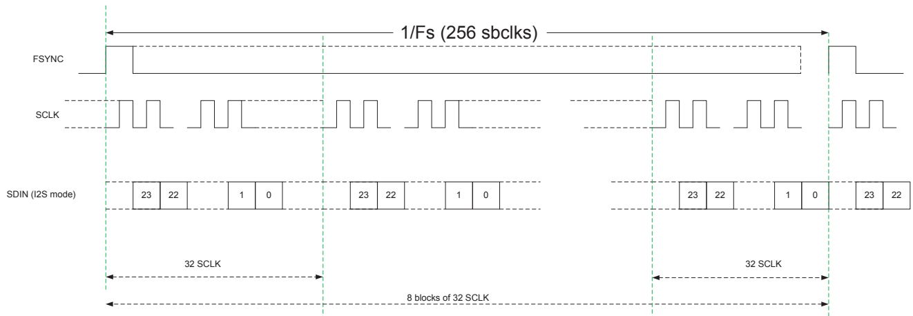
Audio Data Format: TDM8 mode
