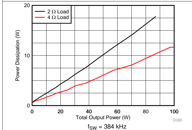
Figure 29. Power Dissipation vs Total Output Power
