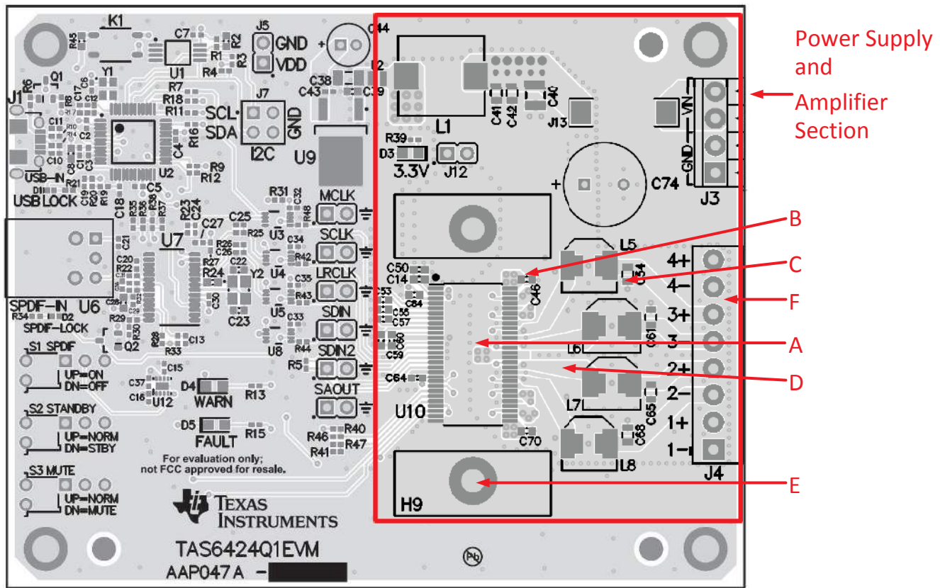
Figure 85. EVM Layout
