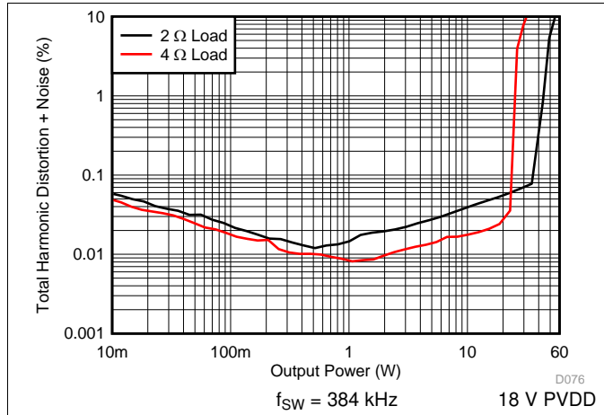
Figure 25. PBTL THD+N vs Power
