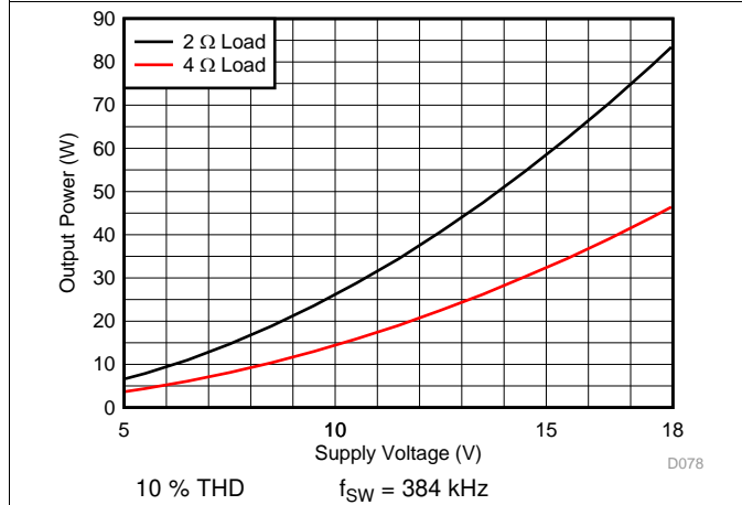
Figure 27. PBTL Output Power vs Voltage
