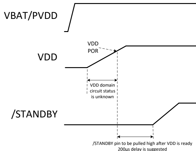
Figure 40. Power-Up Sequence Option 2
