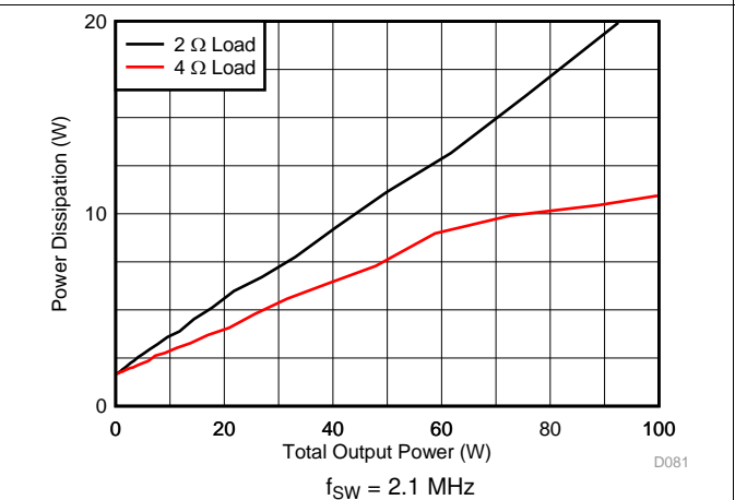
Figure 30. Power Dissipation vs Total Output Power
