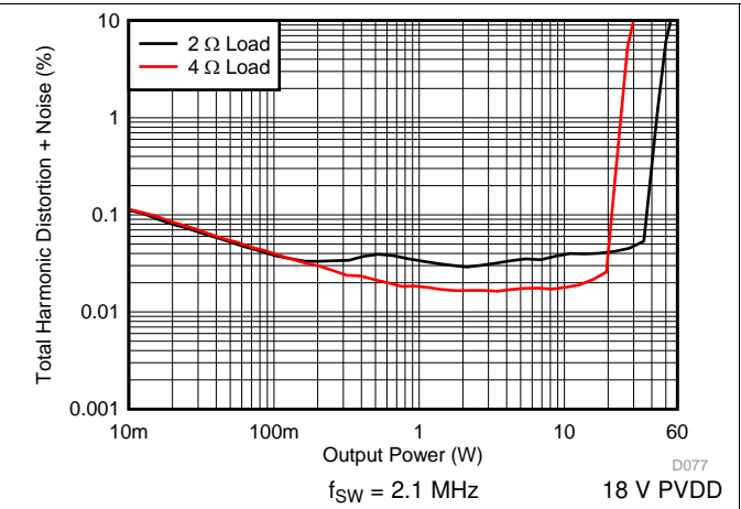
Figure 26. PBTL THD+N vs Power
