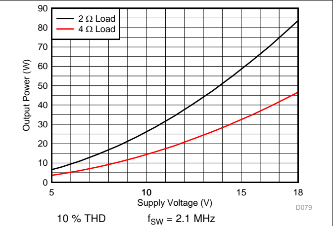
Figure 28. PBTL Output Power vs Voltage
