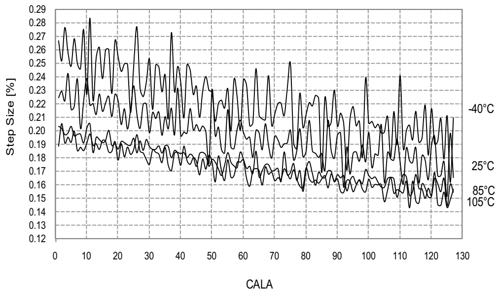
Figure 34-149. 2MHz Internal Oscillator CALA Calibration Step Size
