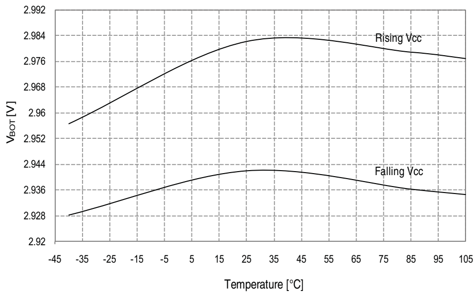
Figure 34-135. BOD Thresholds vs. Temperature
