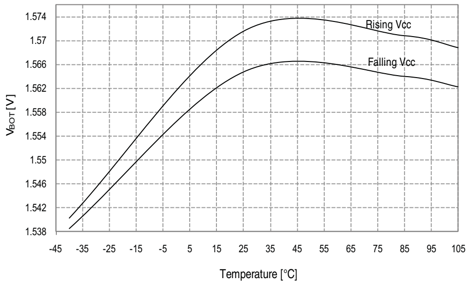
Figure 34-135. BOD Thresholds vs. Temperature
