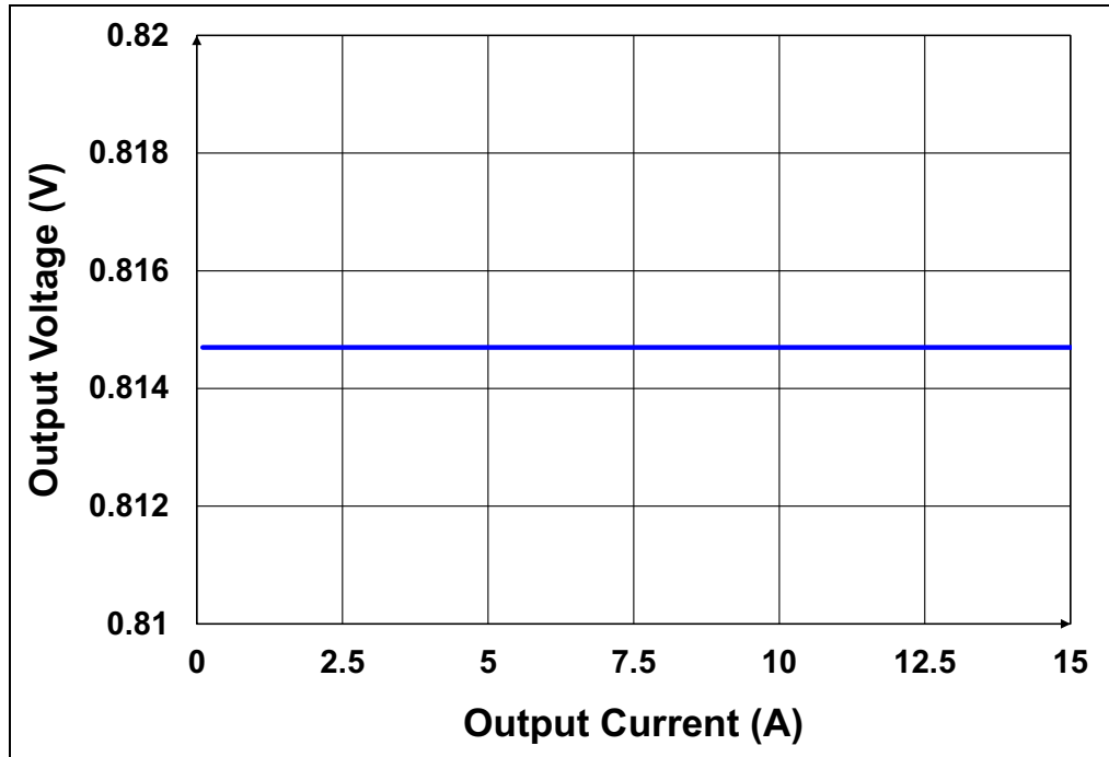
FIGURE C-12: Output Voltage vs. Output Current ( V_{IN} = 30V ).
