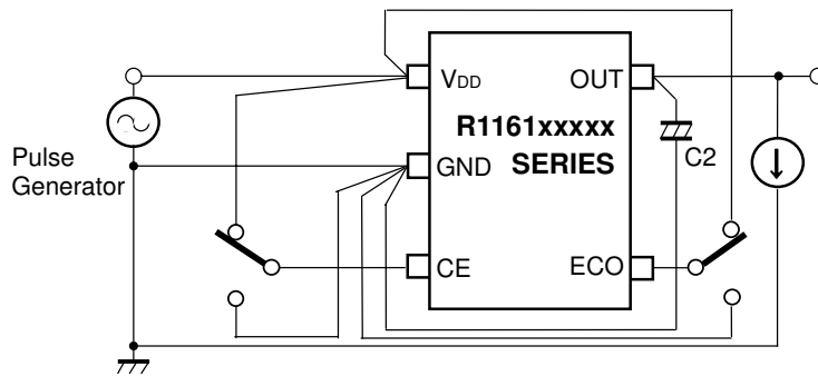
Fig. 7 Ripple Rejection Test Circuit
