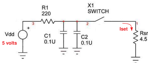
Figure 1 Set Pulse Circuit
