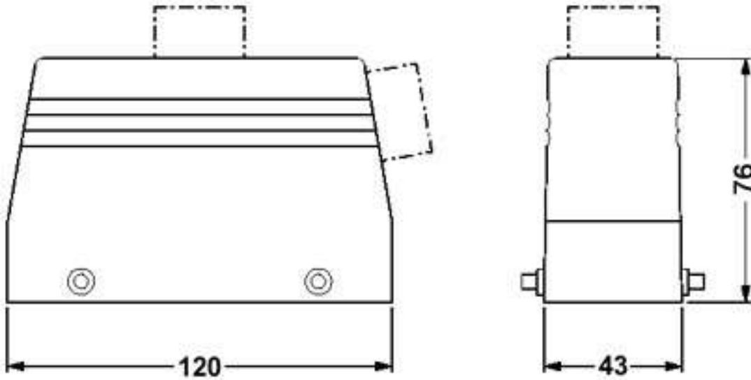
Dimensioned drawing
