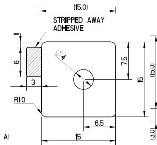
Adhesive Liner View (Bottom)
