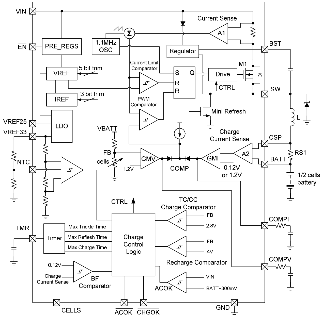
Figure 2—Function Block Diagram
