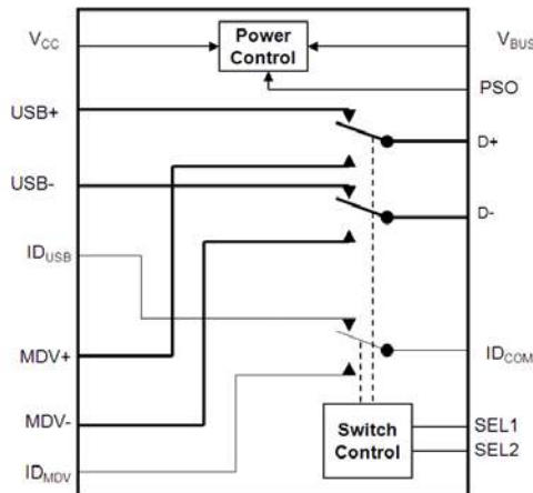
Figure 1. Analog Symbol
