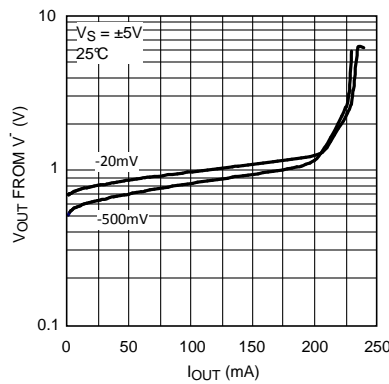
Figure 7. V_{OUT} vs. I_{SINK} (for Various Overdrive)
