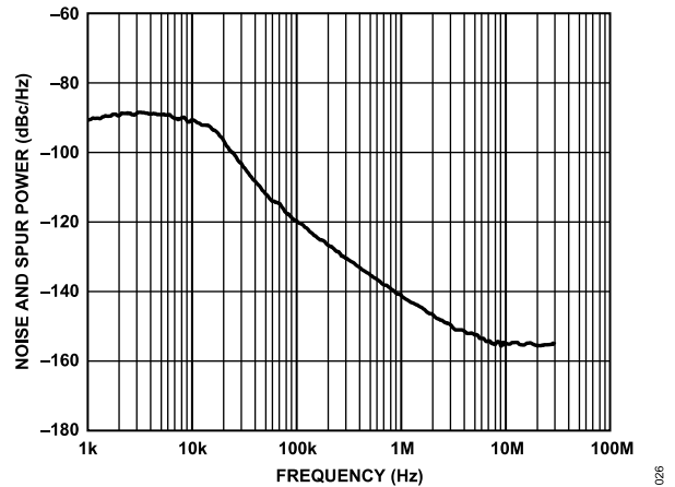
Figure 26. Fractional-N Spur Performance, W-CDMA Band, RF_{OUTA+} = 2113.5 MHz, f_{REFIN} = 122.88 MHz, f_{PFD} = 61.44 MHz, Output Divide by 2 Selected, Loop Filter Bandwidth = 10 kHz, Channel Spacing = 20 kHz
