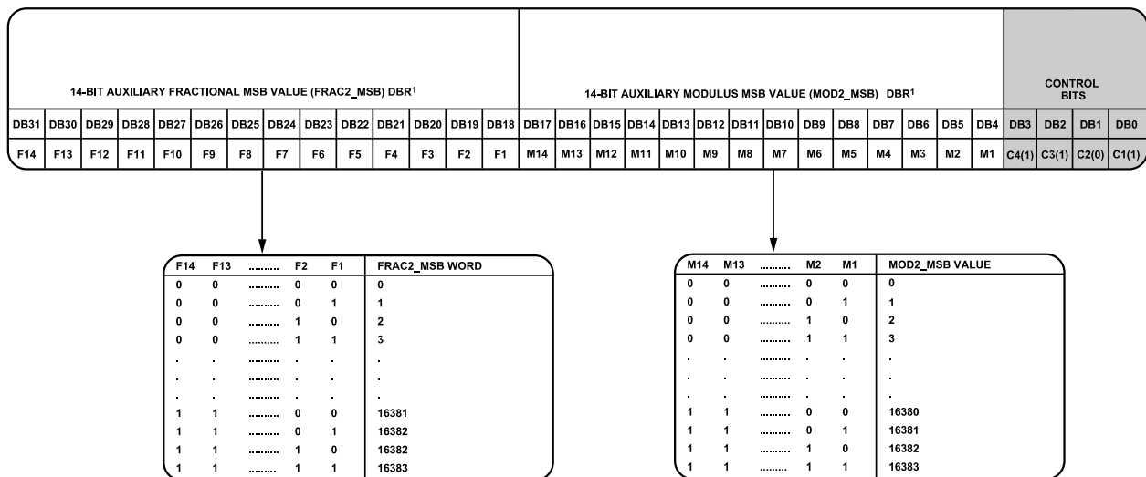
Figure 51. Register 13 Details
