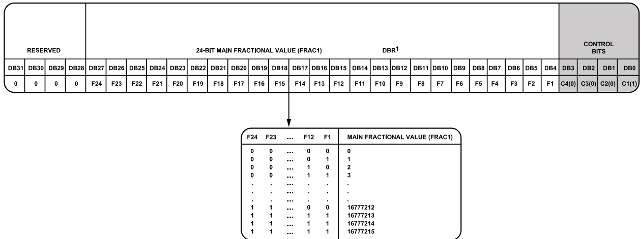
Figure 39. Register 1 Details
