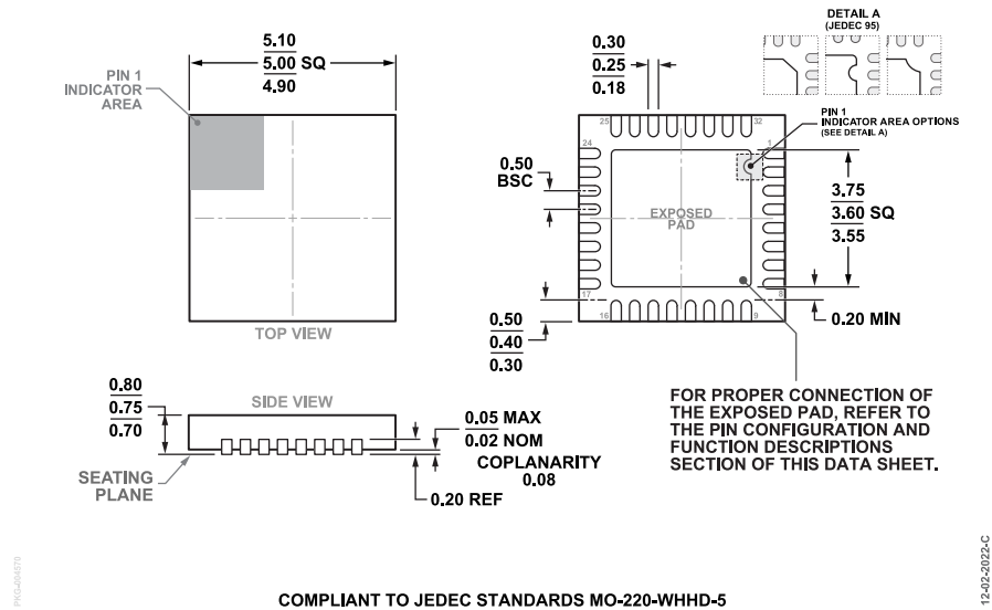
Figure 55. 32-Lead Lead Frame Chip Scale Package [LFCSP] 5 mm × 5 mm Body and 0.75 mm Package Height (CP-32-12) Dimensions shown in millimeters
