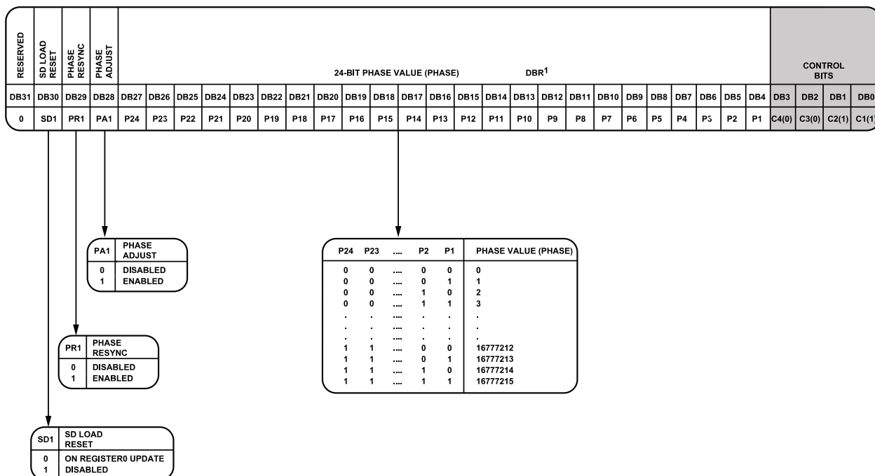
Figure 41. Register 3
