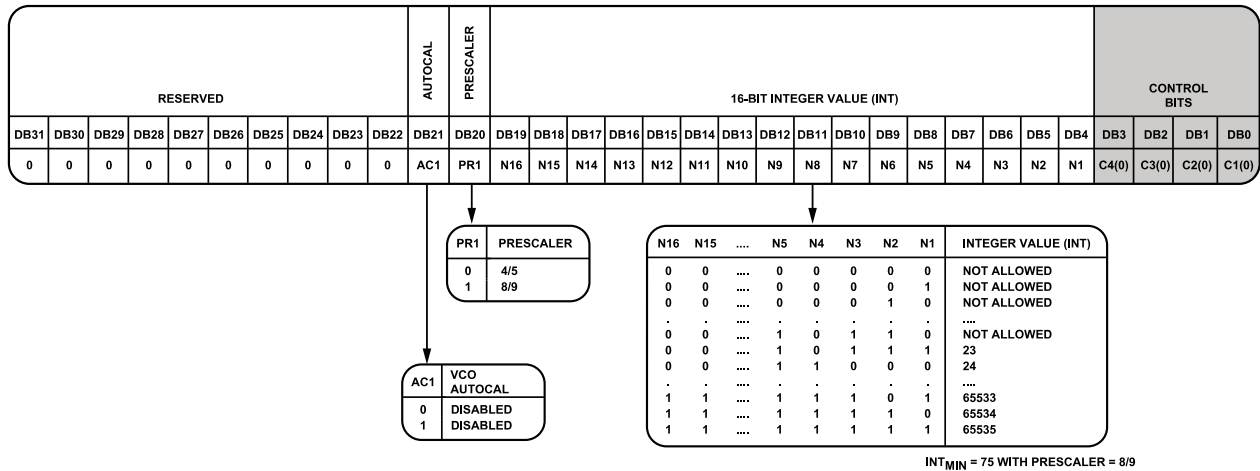
Figure 38. Register 0 Details
