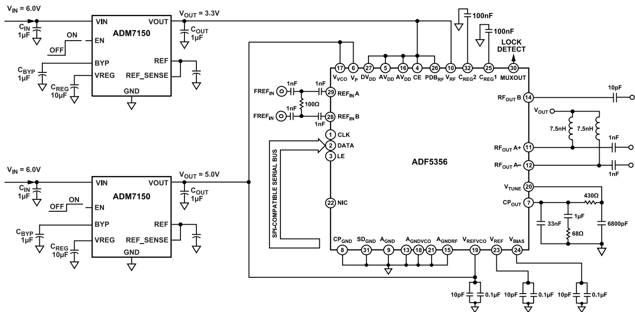
Figure 53. Power Supplies
