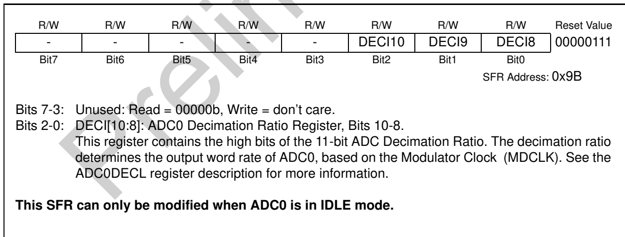
Figure 5.9. ADC0DECH: ADC0 Decimation Ratio Register High Byte
