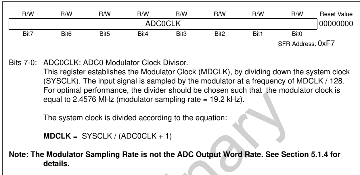
Figure 5.8. ADC0CLK: ADC0 Modulator Clock Divisor
