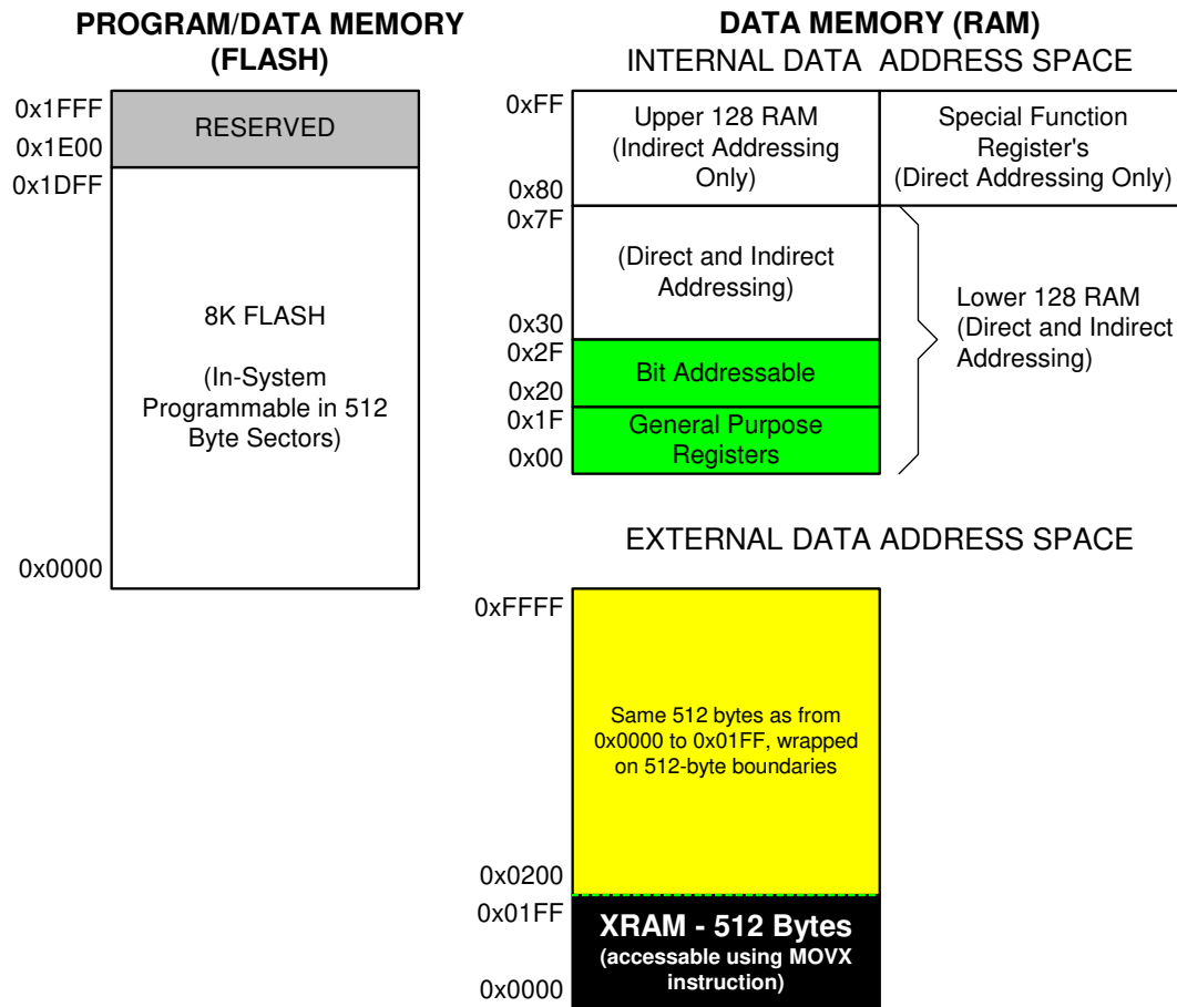
Figure 1.6. Memory Map
