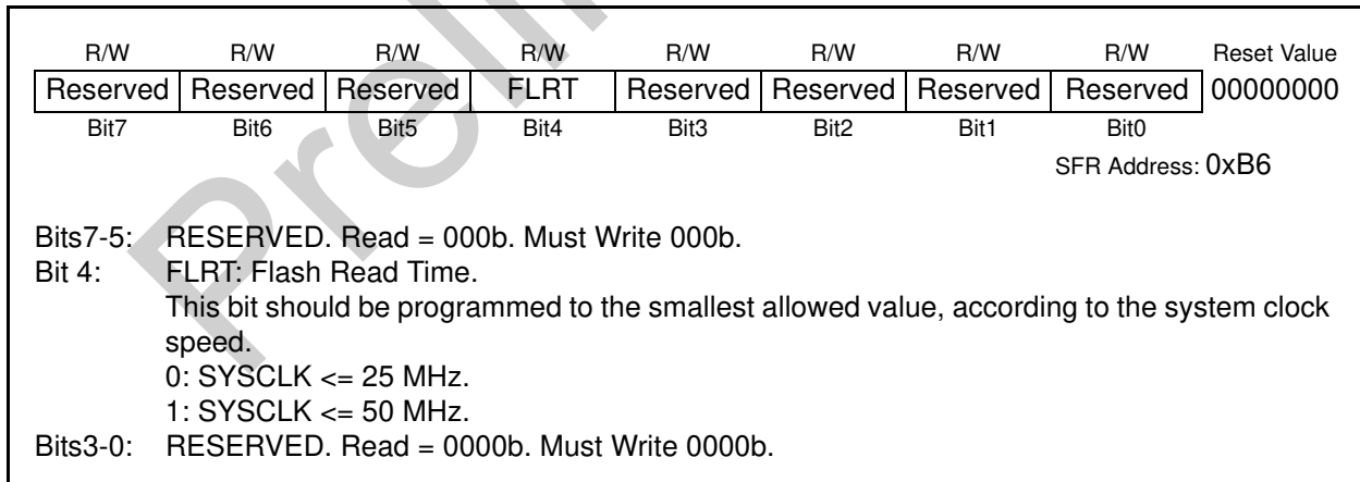
Figure 15.4. FLSC: Flash Scale Register
