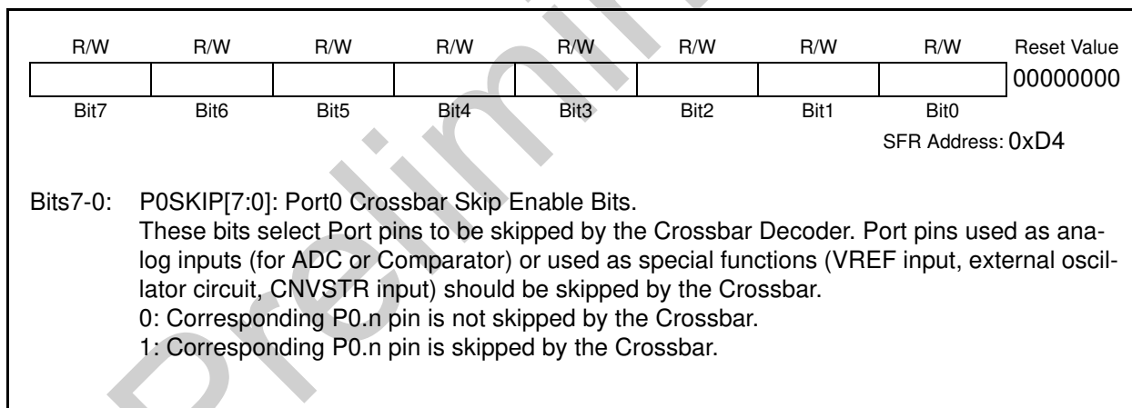
Figure 18.10. P0SKIP: Port0 Skip Register
