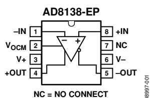
Figure 6. Pin Configuration
