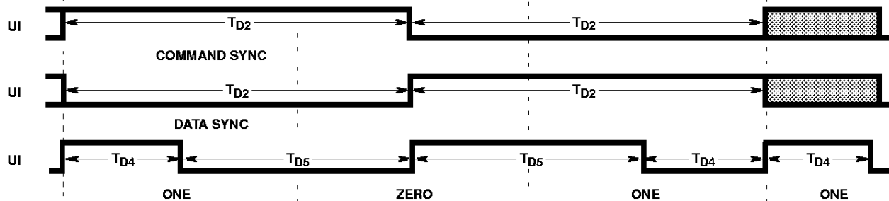
FIGURE 11. DECODER TIMING
