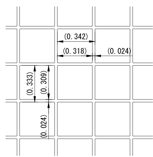
A部拡大図 (50 : 1) A-Portion Magnified Drawing (50:1)
