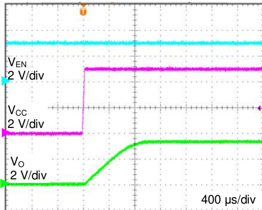
Figure 12. VCC Rise Response ( T_a = +125\text{ }^\circ\text{C} )
