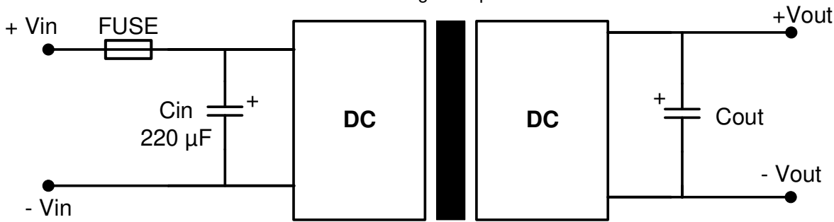
Single Output
