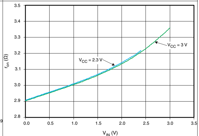
Figure 4. r_{on} vs V_{IN} ( I_{OUT} = -15 mA)
