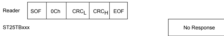
Figure 52. Reset_to_inventory frame exchange between reader and ST25TB512-AC
