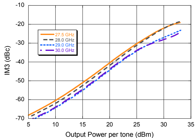
IM3 vs. Output Power per Tone
