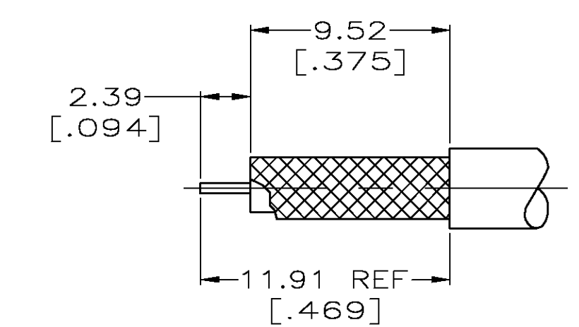
RECOMMENDED STRIP LENGTH SCALE 4:1 (FOR 413589-5 AND 1-413589-2 ONLY)
