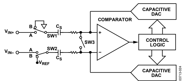
Figure 15. ADC Conversion Phase
