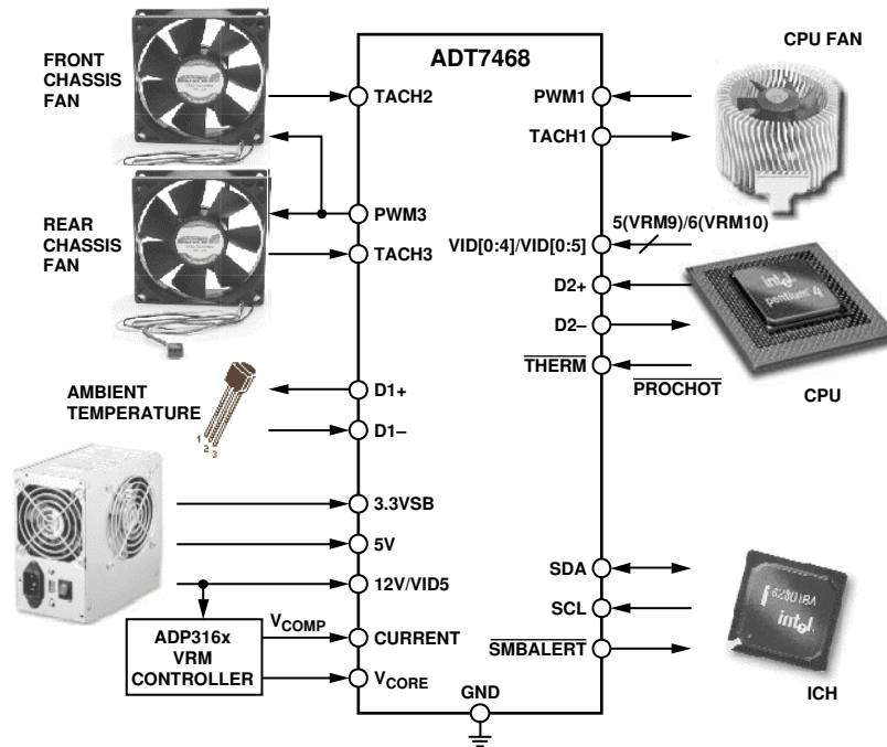
Figure 15. ADT7468 Configuration
