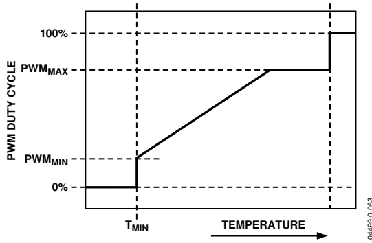
Figure 61. PWM_{MAX} Determines Maximum PWM Duty Cycle Below the T_{THERM} Temperature Limit
