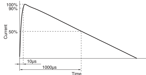
*2 10/1000μs test waveform
