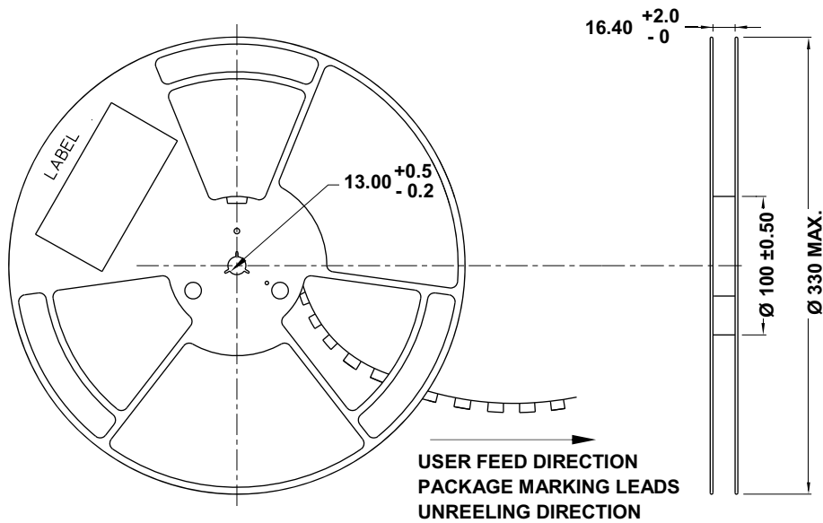
Figure 12: Reel Dimensions
