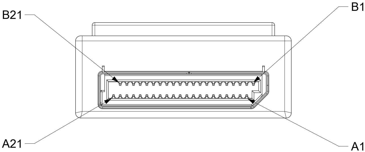
VIEW FROM MATING END OF CONNECTOR
