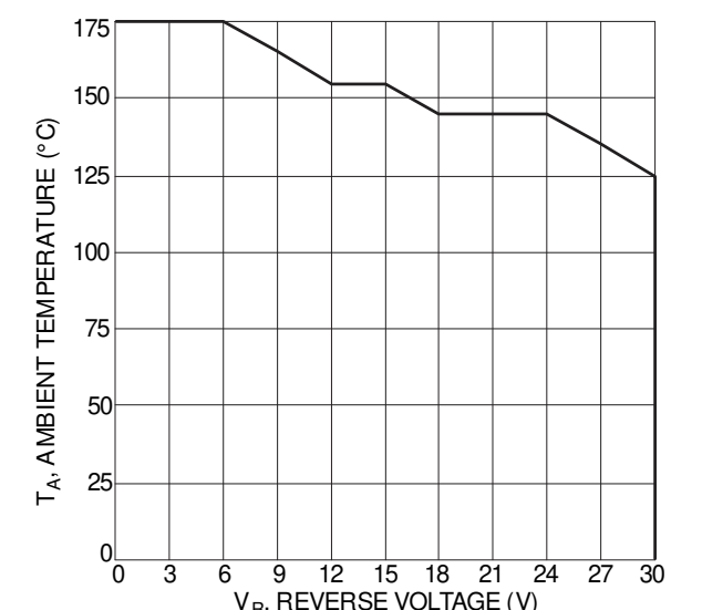
Figure 6 Reverse Voltage Derating
