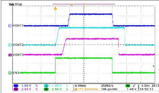
Figure 9-28. Automatic Power Sequencing, MODE = EN1 = HIGH, EN2 = LOW
