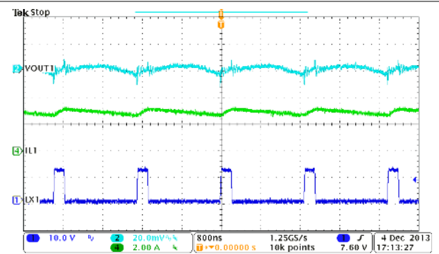
Figure 9-9. Buck1, Steady State Operation at Full Load
