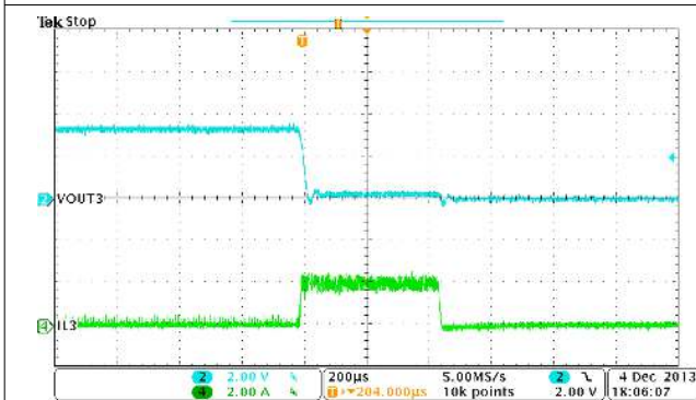
Figure 9-24. Buck3, OCP
