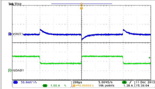
Figure 9-14. Buck1, Load Transient, 0.75 to 1.5 A SR = 0.25 A/µs
