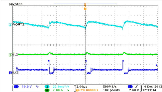
Figure 9-12. Buck3, Steady State Operation at Light Load
