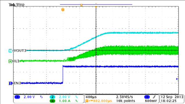
Figure 9-7. BUCK3, Soft-Start With Full Load
