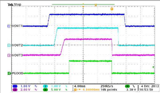
Figure 9-27. Automatic Power Sequencing, MODE = EN1 = EN2 = HIGH
