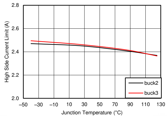
Figure 7-22. Buck2, 3 High-Side Current Limit vs Temperature
