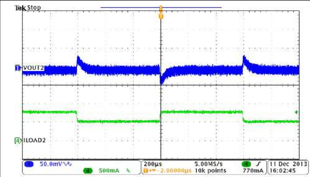
Figure 9-17. Buck2, Load Transient, 0.5 to 0.75 A SR = 0.25 A/µs
