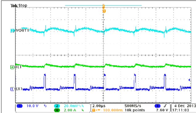
Figure 9-8. Buck1, Steady State Operation at Light Load
