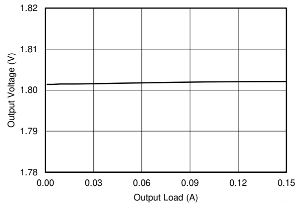
Figure 7-10. LDO2, Load Regulation
