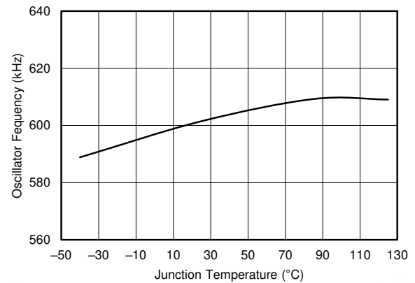
Figure 7-14. Oscillator Frequency vs Temperature
