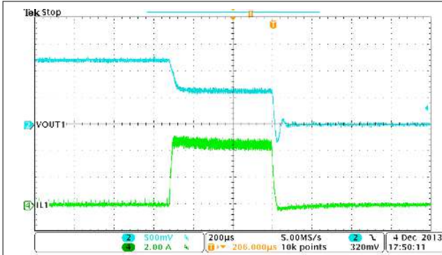
Figure 9-20. Buck1, OCP
