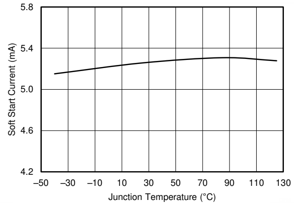
Figure 7-20. SS Pin Charge Current vs Temperature
