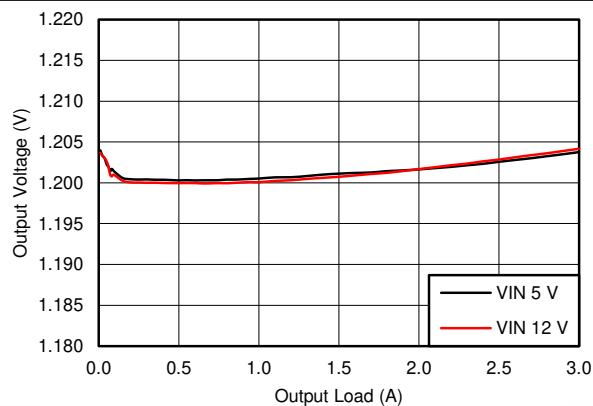
Figure 7-3. BUCK1, Load Regulation
