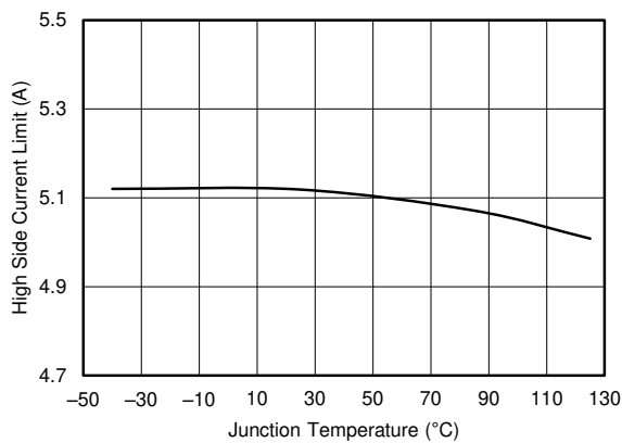
Figure 7-21. Buck1 High-Side Current Limit vs Temperature
