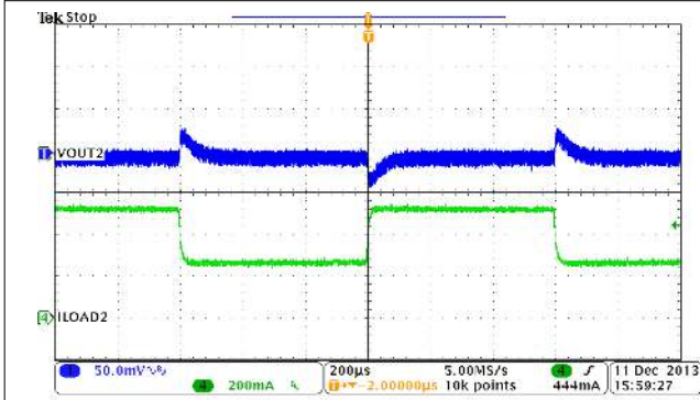
Figure 9-16. Buck2, Load Transient, 0.25 to 0.5 A SR = 0.25 A/µs
