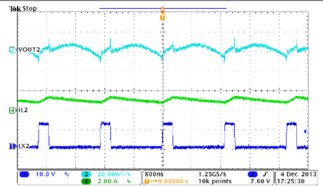
Figure 9-11. Buck2, Steady State Operation at Full Load
