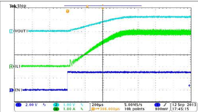
Figure 9-3. BUCK1, Soft-Start With Full Load
