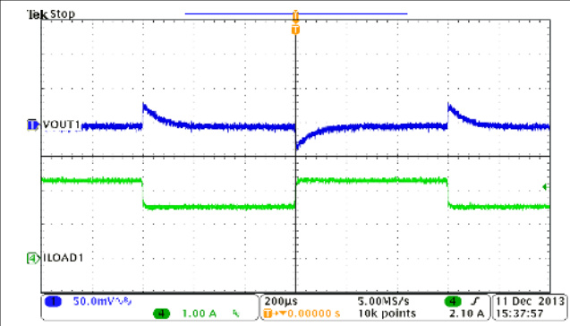
Figure 9-15. Buck1, Load Transient, 1.5 to 2.25 A SR = 0.25 A/µs
