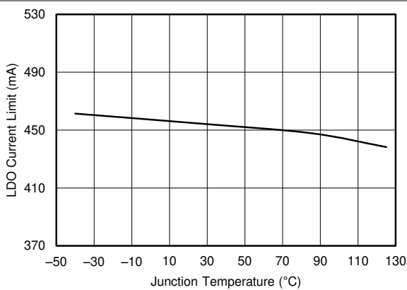
Figure 7-23. LDO Current Limit vs Temperature
