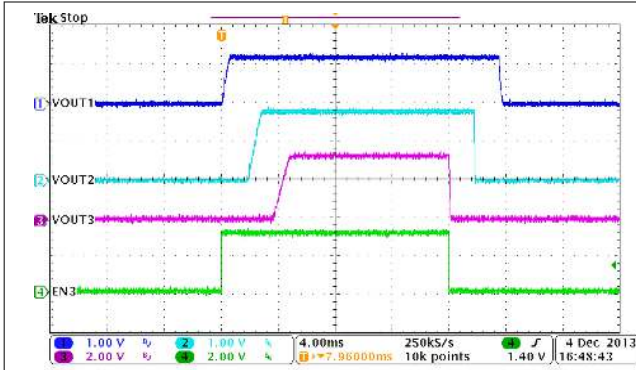
Figure 9-26. Automatic Power Sequencing, MODE = EN1 = EN2 = HIGH
