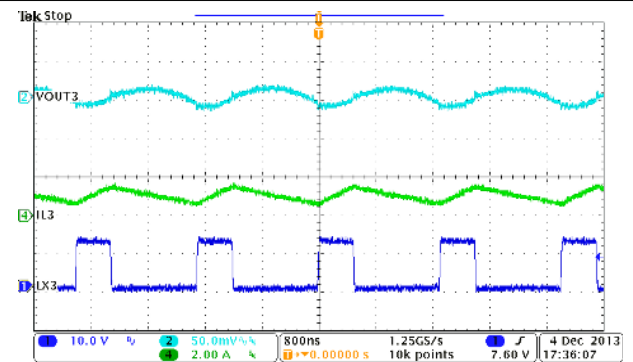
Figure 9-13. Buck3, Steady State Operation at Full Load
