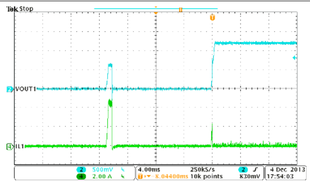
Figure 9-21. Buck1, Hiccup and Recovery
