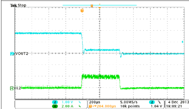
Figure 9-22. Buck2, OCP
