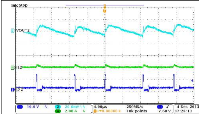
Figure 9-10. Buck2, Steady State Operation at Light Load
