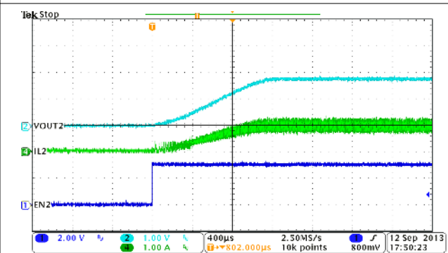
Figure 9-5. BUCK2, Soft-Start With Full Load
