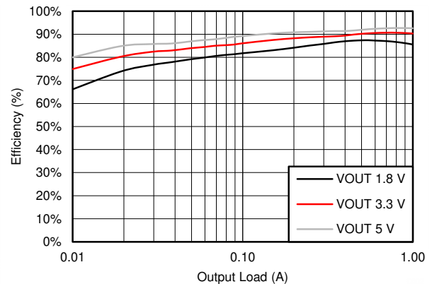
Figure 7-2. BUCK2 Efficiency
