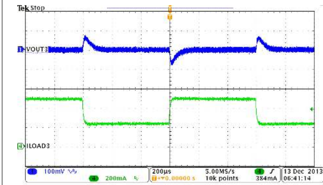
Figure 9-18. Buck3, Load Transient, 0.25 to 0.5 A SR = 0.25 A/µs
