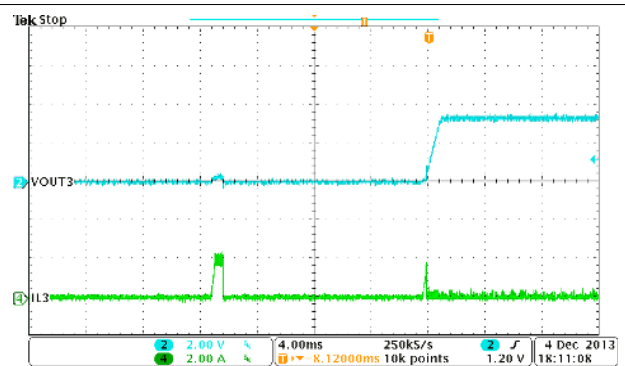
Figure 9-25. Buck3, Hiccup and Recovery
