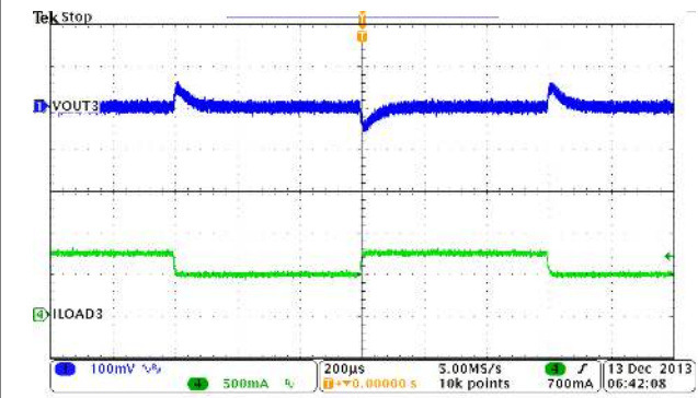
Figure 9-19. Buck3, Load Transient, 0.5 to 0.75 A SR = 0.25 A/µs
