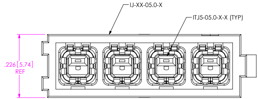
FIG 3 (IJ5-04-05.0-X-S-X SHOWN) (NO GUIDE POST - SEE NOTE 4) (SAME AS FIG 1 EXCEPT AS SHOWN)
