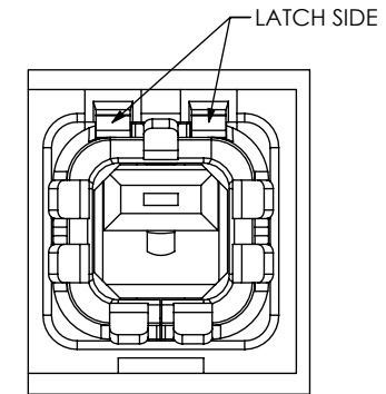
DETAIL 'F' SCALE 8 : 1
