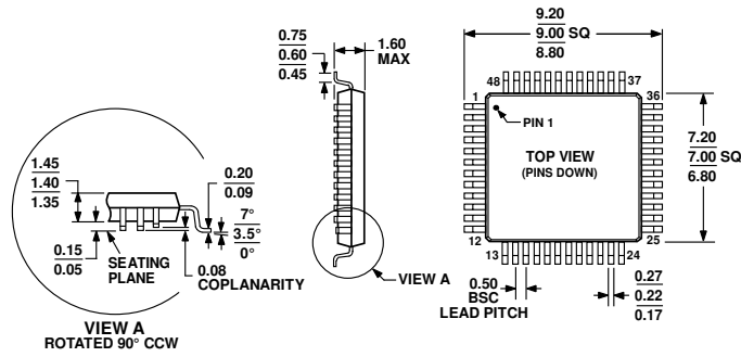
COMPLIANT TO JEDEC STANDARDS MS-026-BBC Figure 13. 48-Lead Low Profile Quad Flat Package [LQFP] (ST-48) Dimensions shown in millimeters
