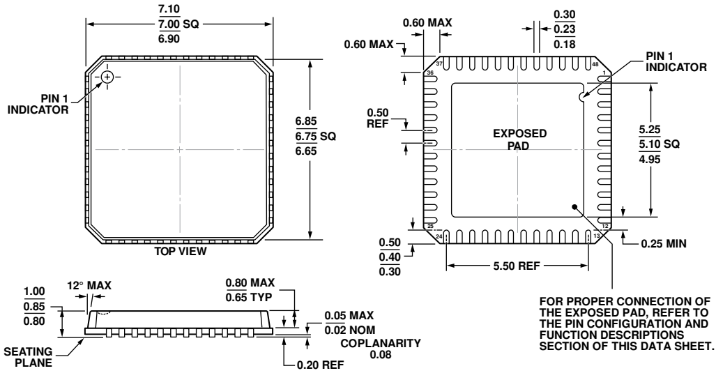
COMPLIANT TO JEDEC STANDARDS MO-220-VKGD-2 Figure 14. 48-Lead Lead Frame Chip Scale Package [LFCSP] 7 mm x 7 mm Body and 0.85 mm Package Height (CP-48-1) Dimensions shown in millimeters
