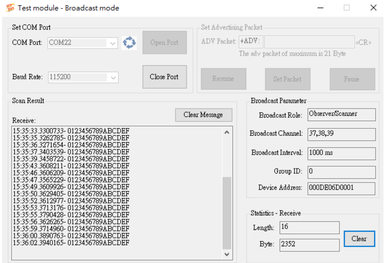
Figure 4-11 receive the advertisement packet
