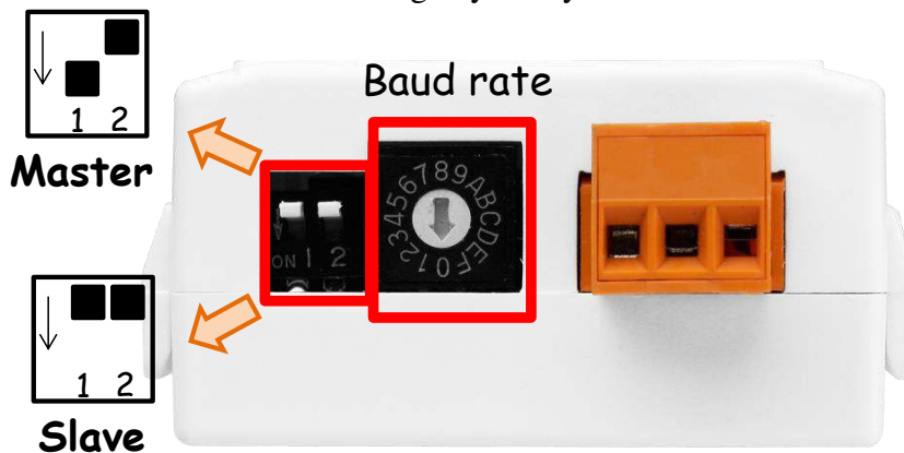
Figure 4-2 change the role, connection mode and baud rate
