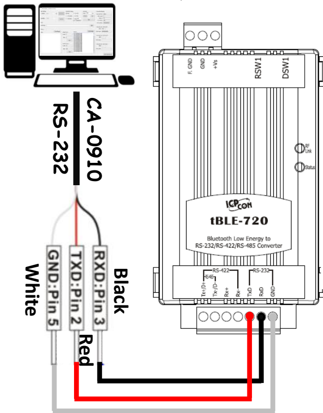
Figure 4-4-1 the architecture of test
