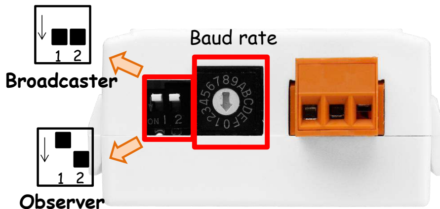
Figure 4-7 change the role, connection mode and baud rate
