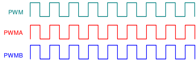
FIGURE 9. SYNCHRONOUS MODE'S OPERATIONAL WAVEFORMS (EN_SYNC = 60% * V CC )
