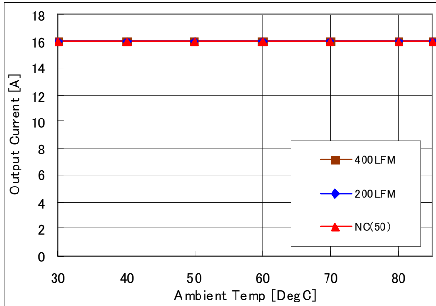
Fig-2.5V-1: Available load current vs. ambient temperature and airflow rates for Vout=2.5V with Vin=12.0V. Maximum component temperature ≤ 120°C
