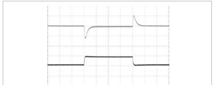
Output disabled by removing V_i at: T_{P1} = +25^{\circ}\text{C} , V_i = 48\text{ V} , I_o = 1\text{ A} electronic load. Top trace: output voltage (5 V/div.). Bottom trace: input voltage (20 V/div.). Time scale: (1 ms/div.).
