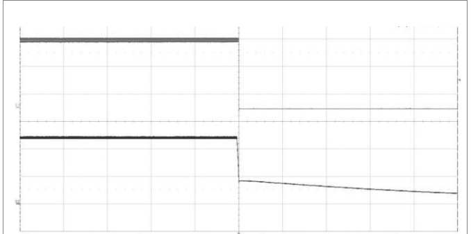
Shut-down enabled by disconnecting V_I at: T_{P1} = +25^\circ\text{C} , V_I = 48\text{ V} , I_O = 6\text{ A} resistive load. Top trace: output voltage (2 V/div.). Bottom trace: input voltage (20 V/div.). Time scale: (200 ms/div.).
