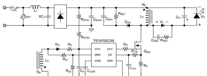
Buck-Boost Converter
