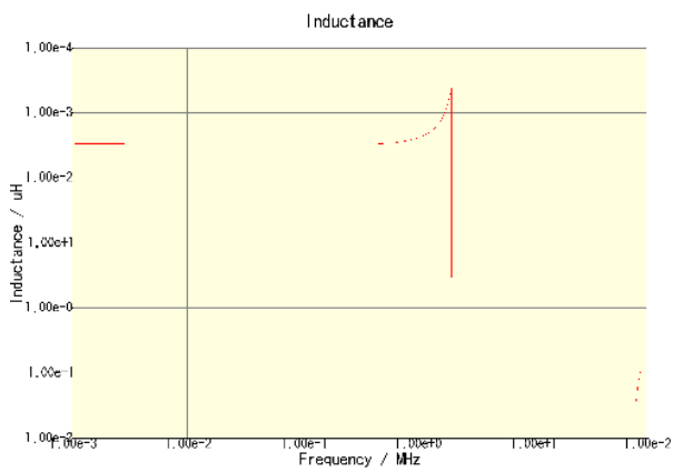
CLF6045T-331M-CA
