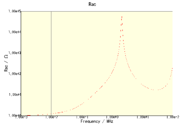
CLF6045T-331M-CA
