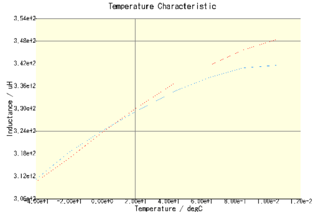
CLF6045T-331M-CA(DC = 0A)
