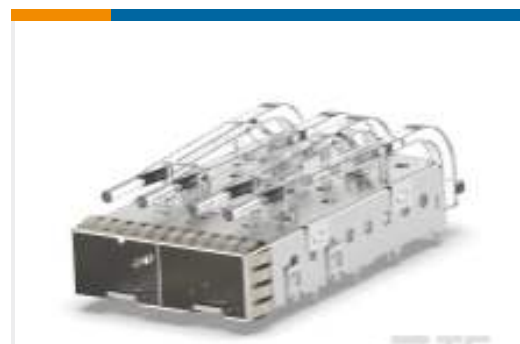
TE Part #2007262-2 SFP+ 1x2 Cage Assembly, Light
