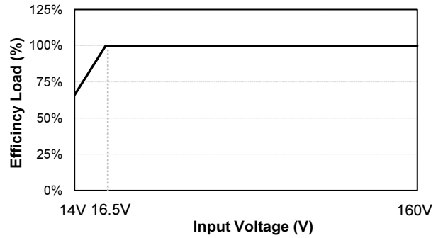
Typical Derating Curve VS Input Voltage
