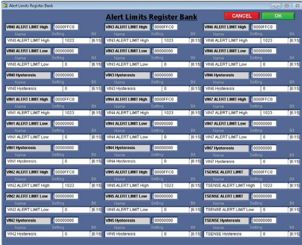
Figure 26. Alert Limits Register Bank Window
