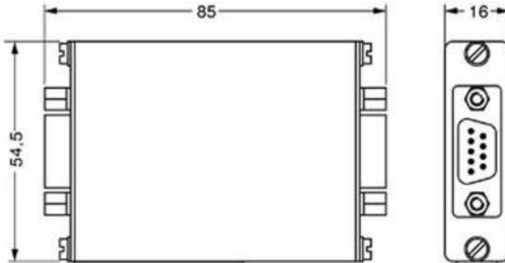
Dimensioned drawing
