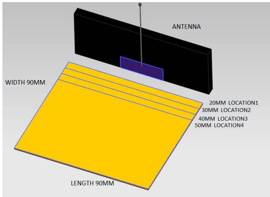
FIGURE 4.1 FOUR LOCATIONS WITH VERTICAL GROUND
