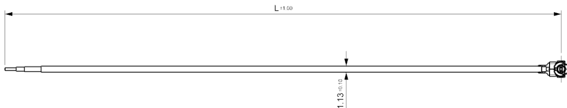
FIGURE 2. CABLE LINE VIEW OF CELLULAR QUAD BAND FLEX ANTENNA
