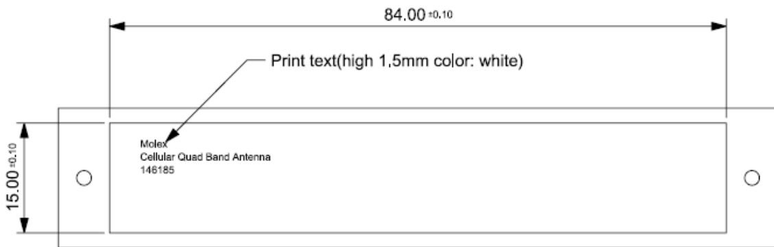
FIGURE 1. DIMENSION OF CELLULAR QUAD BAND FLEX ANTENNA
