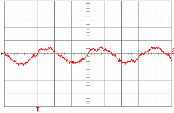
Fig. 17: Input reflected ripple current, i_s (10 mA/div), measured through 10 \mu H at the source at full rated load current and V_{in} = 56 V. Refer to Fig. I for test setup. Time scale: 1 \mu s/div.
