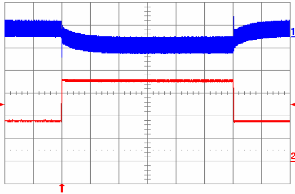
Fig. 9: Output voltage response to load current step-change (3.5 A – 7 A – 3.5 A) at V_{in} = 56 V. Top trace: output voltage (200 mV/div.). Bottom trace: load current (2 A/div). Bottom trace: load current (5 A/div.). Current slew rate: 5 A/ \mu s. C_o = 1 \mu F ceramic. Time scale: 0.5 ms/div.
