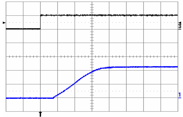
Fig. 8: Turn-on transient at full rated load current (resistive) plus 2,200 µF at V_{in} = 56\text{ V} , triggered via ON/OFF pin. Top trace: ON/OFF signal (5 V/div.). Bottom trace: output voltage (5 V/div.). Time scale: 2 ms/div.
