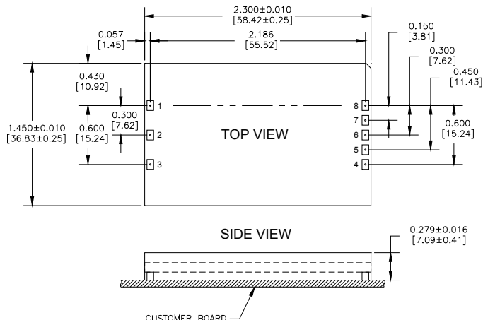
QM48S (Surface-mount)
