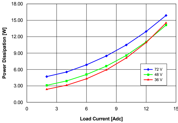
Fig. 5: Power dissipation vs. load current and input voltage for converter mounted vertically with air flowing from pin 3 to pin 1 at a rate of 300 LFM (1.5 m/s) and T_a = 25^\circ\text{C} .
