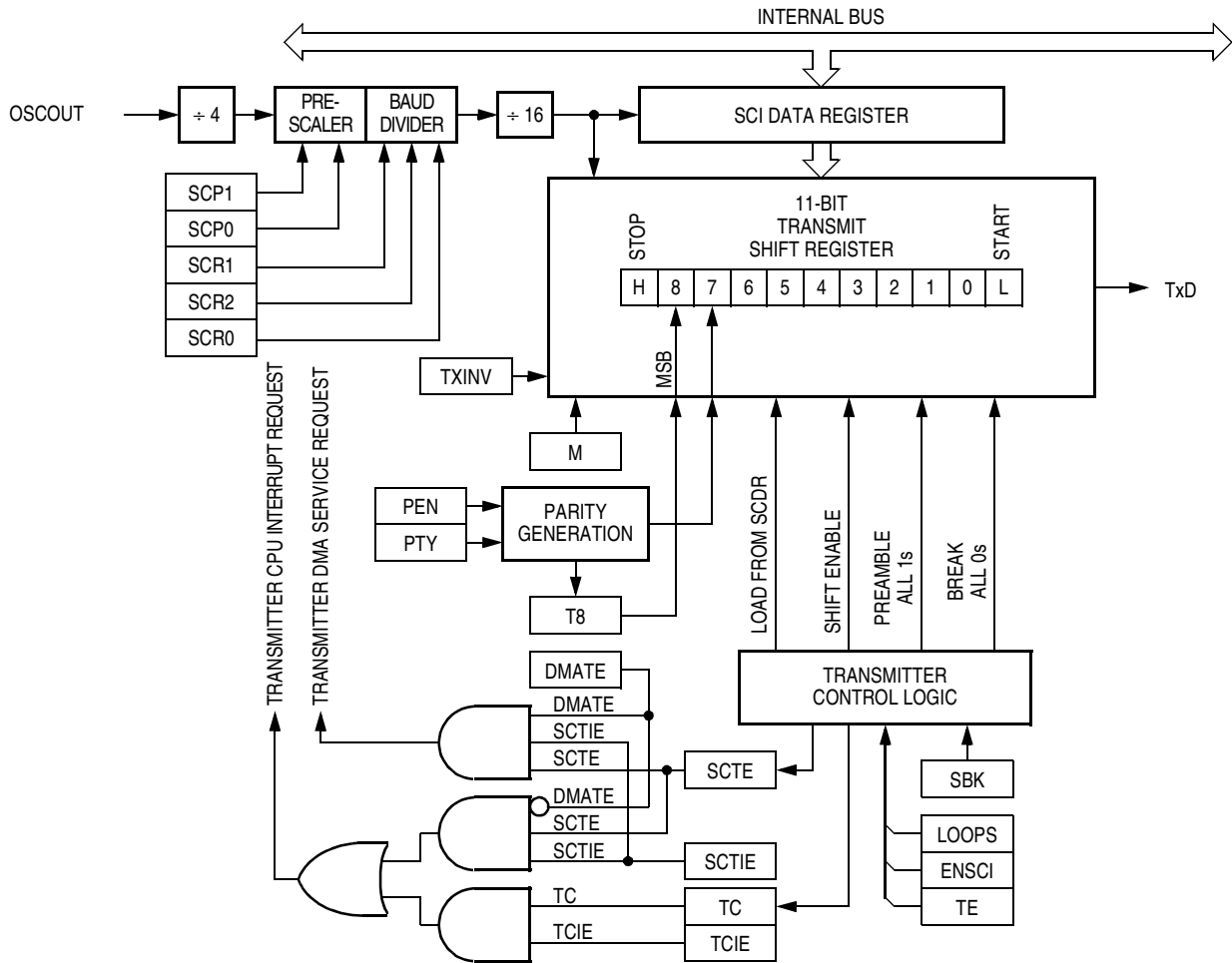
Figure 11-4. SCI Transmitter
