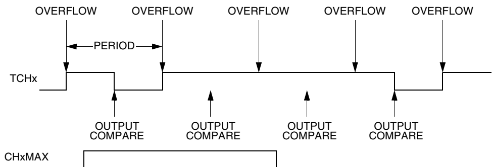
Figure 10-11. CHxMAX Latency
