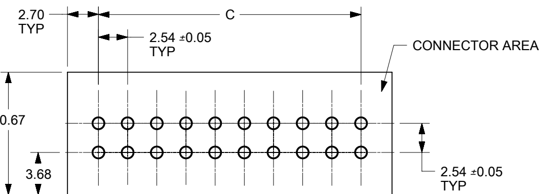
PCB LAYOUT: COMPONENT SIDE 2.36 THICK PCB
