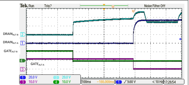
Figure 10-9. 4-Pair Single Signature Class 0-4 Disconnect
