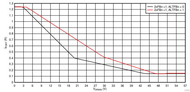
Figure 9-57. 2x Mode (2xFBn = 1) Foldback Curves, I PORT vs V DRAIN
