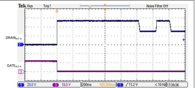
Figure 10-5. 2-Pair Backoff Due to PCut Fault
