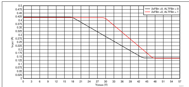
Figure 9-79. 1x Mode (2xFBn = 0) Foldback Curves, I PORT vs V DRAIN
