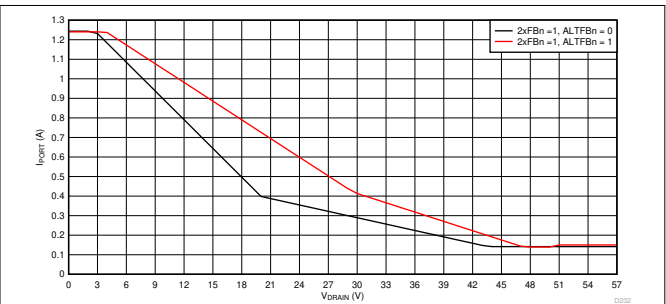
Figure 9-80. 2x Mode (2xFBn = 1) Foldback Curves, I PORT vs V DRAIN
