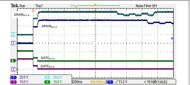
Figure 10-7. 4-Pair Backoff Due to I_{LIM} Fault
