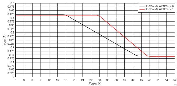
Figure 9-56. 1x Mode (2xFBn = 0) Foldback Curves, I PORT vs V DRAIN
