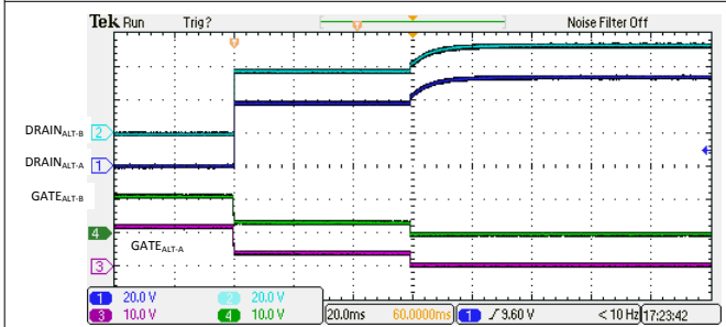
Figure 10-6. 4-Pair I_{LIM} Foldback and Turn Off
