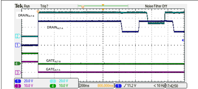
Figure 10-8. 4-Pair Backoff Due to 4PPCut Fault
