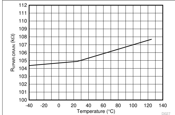
Figure 7-27. R_{\text{OFF}} (VPWR to DRAIN) vs Temperature
