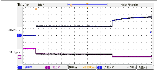
Figure 10-4. 2-Pair I_{LIM} Foldback and Turn-Off
