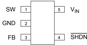
Figure 2. Pin Configuration of AP3015/A (Top View)
