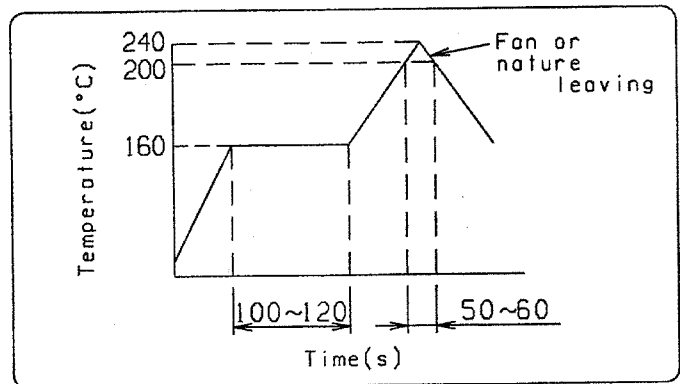
Temperature profile of reflow soldering. (Fig-6)
