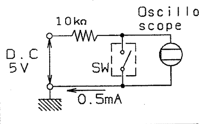
Measurement circuit diagram.(Fig-4)
