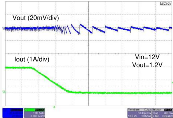
Figure 24. FAN2306 Transition from CCM to DCM
