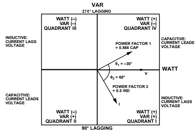
WATT(+) INDICATES POWER RECEIVED (IMPORTED FROM GRID) WATT(-) INDICATES POWER DELIVERED (EXPORTED TO GRID)
