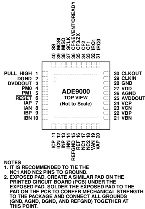
Figure 3. Pin Configuration
