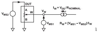
Figure 32. Wiper Resistance
